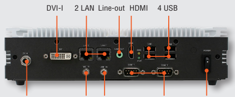
Lockable DC Jack Mic-in Line-in 2 COM Power Switch DVI-I 2 LAN Line-out HDMI 4 USB
