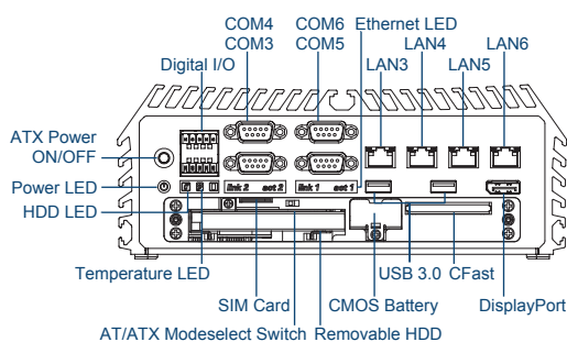
Front Panel
