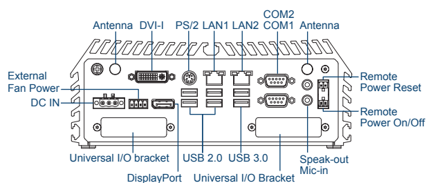
Rear Panel
